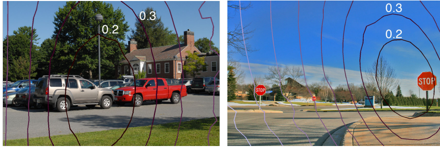
Fig. 9. Shown in each panel are authentic images with superimposed level curves showing the deviation of the estimated principal point from the true principal point as a function of spatial position in the image. The principal point for the left image was determined from the left-most car’s wheels, and for the right image, the known geometry of the stop sign.
